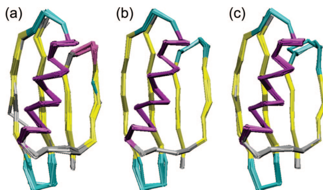
Figure 5. Ensembles of 10 lowest energy structures of GB1 computed with CST restraints: (a) using distances and CST data and variable p offset and p scale ; (b) using distances, CST, TALOS, and VEAN restraints and variable p offset and p scale ; (c) using distances and CST with p scale and p offset fixed to values from the lowest energy structure in (b). The coloring is according to secondary structure (helix in purple, strands in yellow, turns in cyan, and coils in gray).
