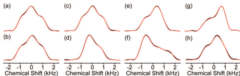
Figure 3. ROCSA experimental and simulated lineshapes. Experimental ROCSA pseudostatic powder patterns (black) are overlaid with the best-fit simulations (red). Sites presented are (a) A26, (b) A48, (c) D36, (d) D47, (e) K28, (f) K50, (g) T25, and (h) T51. Fit values and experimental errors for each site are provided in Table 1.
