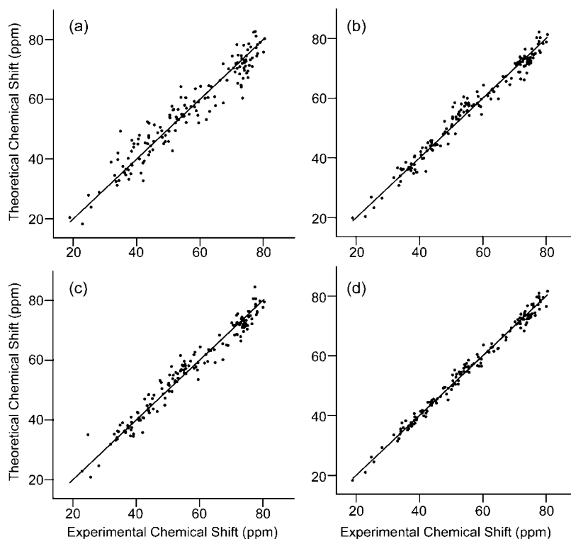
Figure 6. Comparison between experimental and theoretical CST elements, obtained by using different backbone geometries. In all cases, theoretical chemical shielding tensor principal components were converted to chemical shift tensor elements using regression analysis. Backbone geometries represented, as well as R^2 and rmsd, between theory and experiment are (a) structure calculated with distance only (structure 1, Table 3), R^2 = 0.92 , rmsd = 4.4 ppm, (b) 2QMT crystal structure, R^2 = 0.97 , rmsd = 2.5, (c) previously published 47 SSNMR structure of GB1 (structure 10, Table 3, pdb code 2JSV), R^2 = 0.97 , rmsd = 2.9 ppm, and (d) structure solved with calibrated CST data (structure 8) R^2 = 0.99 , rmsd = 1.6 ppm.
