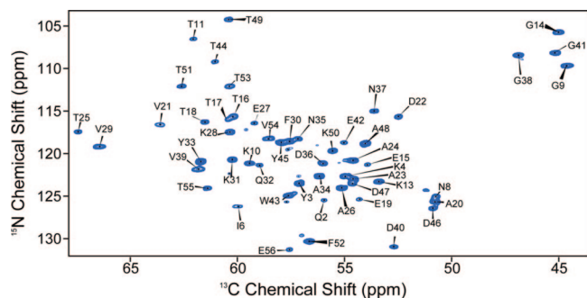
Figure 2. First ^{15}\text{N} – ^{13}\text{C}\alpha plane from the ^{15}\text{N} – ^{13}\text{C} CSA– ^{13}\text{C} 3D experiment. Spectra were acquired and processed with parameters discussed in the Experimental and Computational Methods section. Resonance assignments are based upon published values. 24
