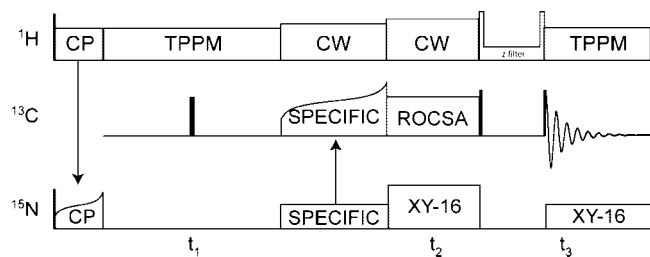
Figure 1. ^{15}\text{N} – ^{13}\text{C} CSA– ^{13}\text{C} 3D ROCSA pulse sequence. Transverse ^{15}\text{N} coherence is created by adiabatic CP from ^1\text{H} , followed by isotropic chemical shift evolution period ( t_1 ) and selective polarization transfer to ^{13}\text{C}\alpha with SPECIFIC-CP. 27 ROCSA 25 recoupling is applied to the ^{13}\text{C} spins, with a coherence filter (including States-TPPI hypercomplex sampling) prior to acquisition. During ^{13}\text{C} ROCSA, ^1\text{H} was decoupled with a CW field ( \sim 125 kHz nutation frequency) and ^{15}\text{N} with rotor-synchronized \pi -pulses of 10\ \mu\text{s} with XY-16 supercycling.
