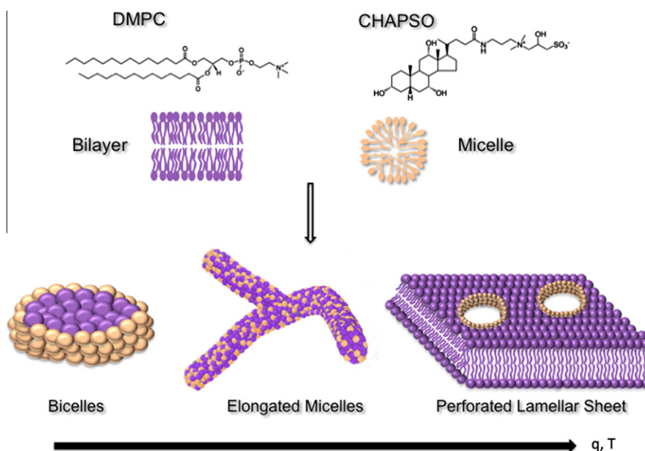
Fig. 1. Phase behavior of bicellar mixtures. Bicelles are formed by mixing a phosphatidylcholine lipid such as DMPC with a detergent such as CHAPSO. The detergent shields the hydrophobic edges of the bilayer. With increasing temperatures and q , disc-shaped bicelles undergo phase transformation into worm-like cylindrical micelles and perforated lamellar sheet, which may also be beneficial for crystallization.
