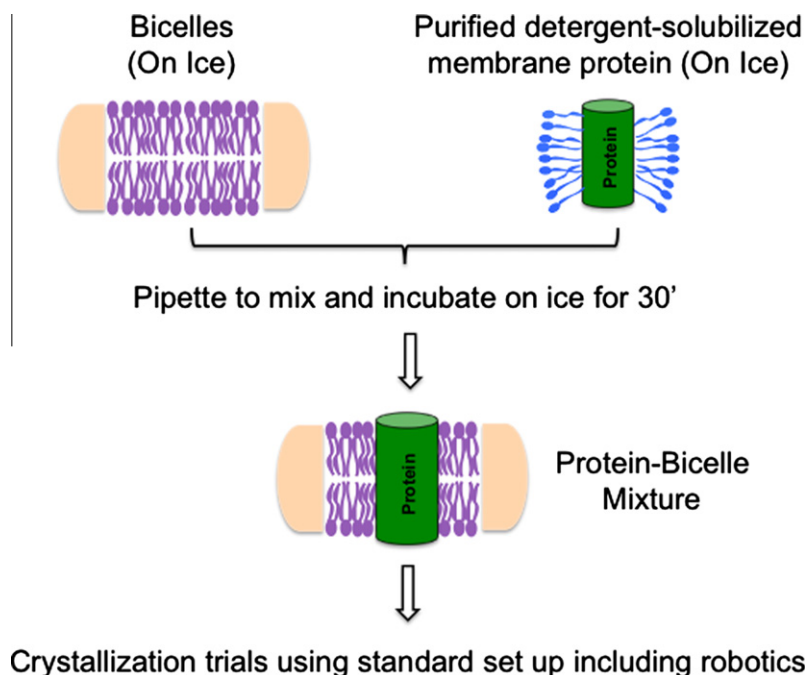
Fig. 2. Bicelle crystallization. Detergent-solubilized purified membrane proteins can be mixed directly with bicelles on ice. Homogenous mixing can be achieved by simply pipetting the contents up and down. After incubating the protein/bicelle mixture on ice for ~30 min, crystallization trials can be carried out using any standard format including robotics.
